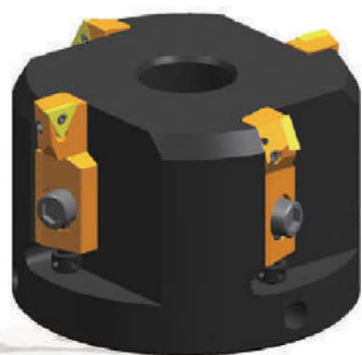
• STOP FACE SEALING CRANK SHAFT BORING TOOL
